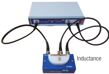
構成例(Bode 100, B-WIC)
